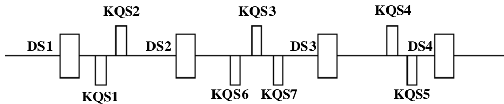
Figure 16.3 Four-bend achromat schematic layout
