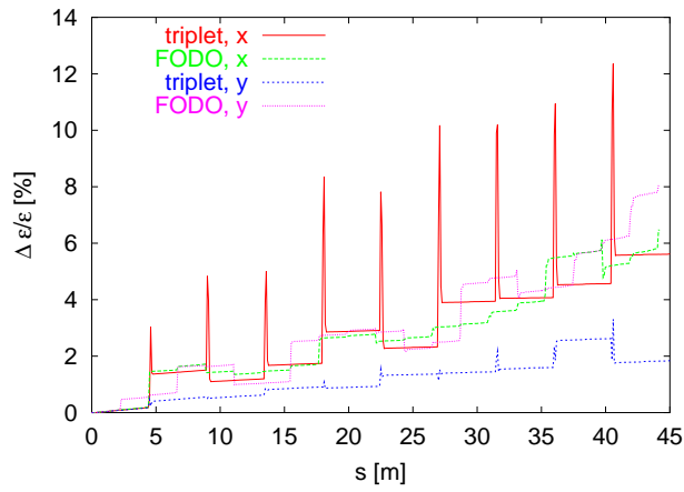
Figure 10.18 The emittance growth along the linac for the FODO and the triplet lattice. A local variation of the gradient with an amplitude of \Delta\epsilon=5\% is assumed.
