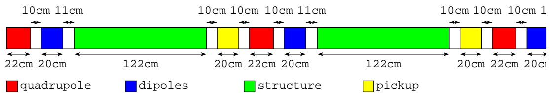
Figure 10.4 Sketch of a single cell in the FODO lattice.
