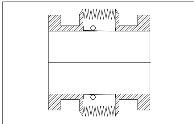
Figure 24.4 RF screened bellow.
