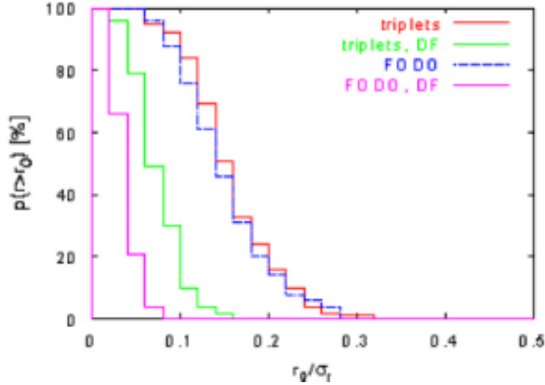
Figure 10.22 Energy dispersion in the FODO lattice and the triplet lattice. A beam was accelerated with a beam loading 10 % smaller than nominal, the relative offset to the nominal beam is plotted normalised to the final beam sizes. The plot shows the result if only one-to-one correction is applied and after the use of dispersion free steering.
