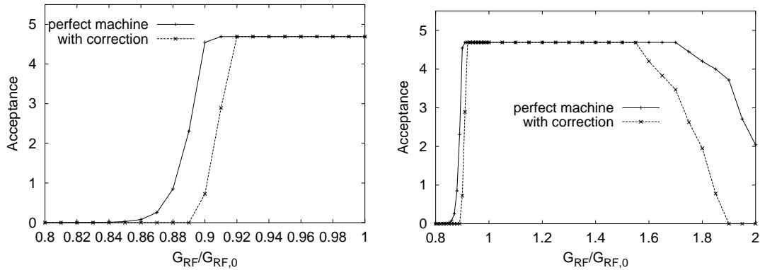
Figure 10.19 The acceptance of the triplet lattice (set number 2) as a function of the gradient error. In one case a perfectly aligned machine is assumed. In the other case the smallest acceptance of 100 different machines is plotted. These machines had initial position errors for all elements and were corrected using one-to-one correction.
