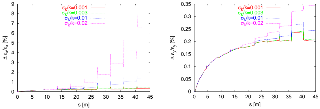
Figure 10.21 The chromatic emittance growth in the triplet lattice for different errors in the quadrupole strengths. The left plot shows the horizontal, the right one the vertical plane.
