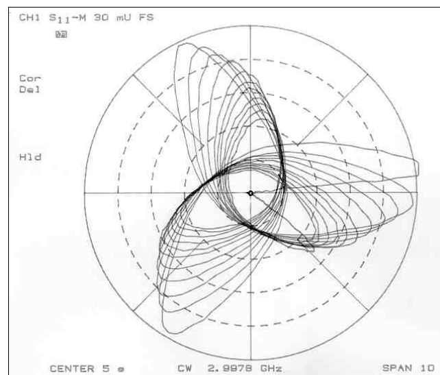
Figure 9.4 Bead-pull measurement: an error of about 40 ° between the 1 st and last cell is measured in this reflection diagram, corresponding to a phase slip of \pm 10^\circ between electron and wave over 32 cells. The loss in accelerating efficiency is less than 1 %. The cells are not equipped with dimple tuners.
