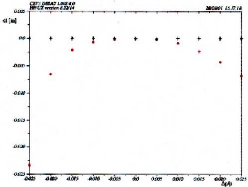
Figure 14.5 Off-energy Particles Longitudinal Position at DL Input (Crosses) and Output (Dots) First Order Correction
