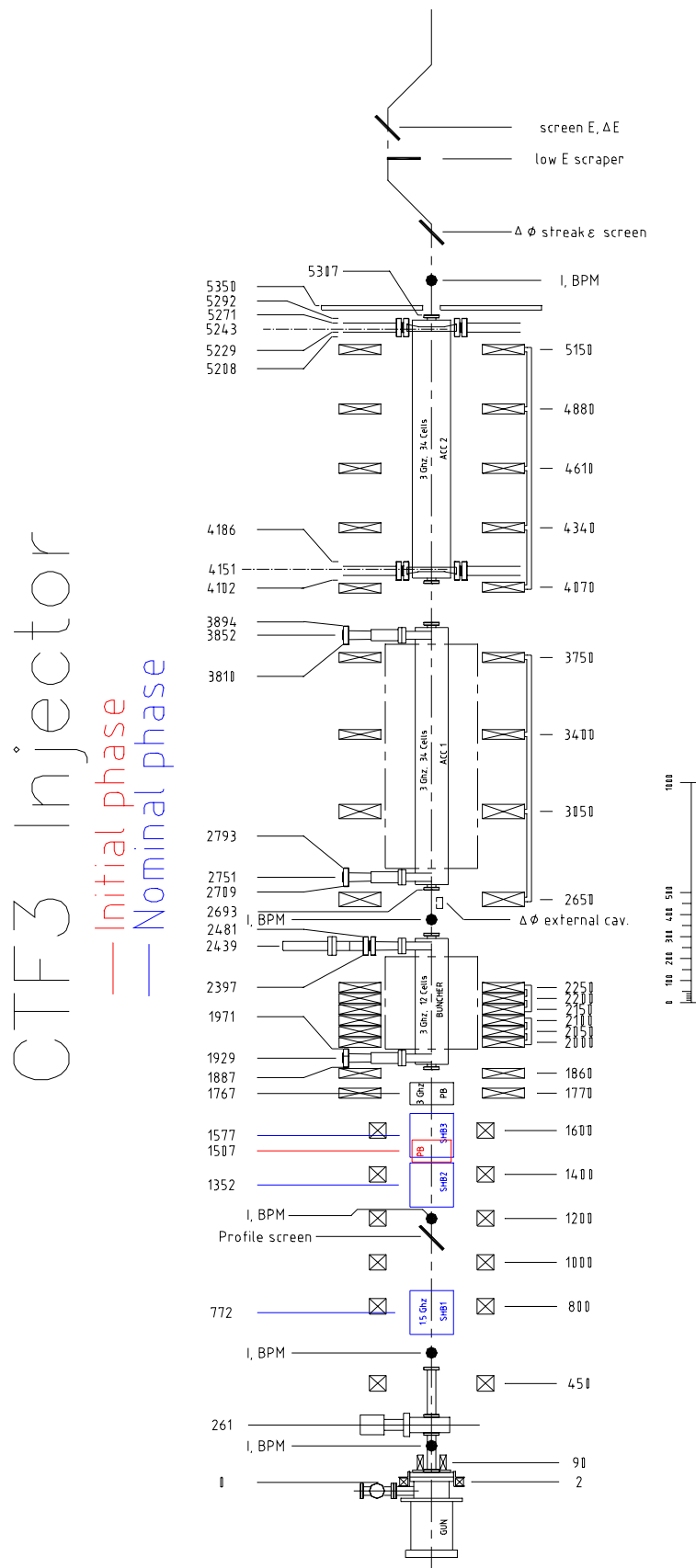
Figure 7.2 CTF3 Nominal Phase Injector block diagram.
