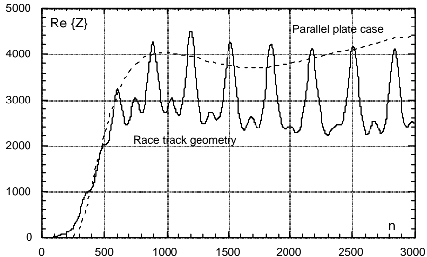
Figure 13.1 Real part of the CSR impedance
