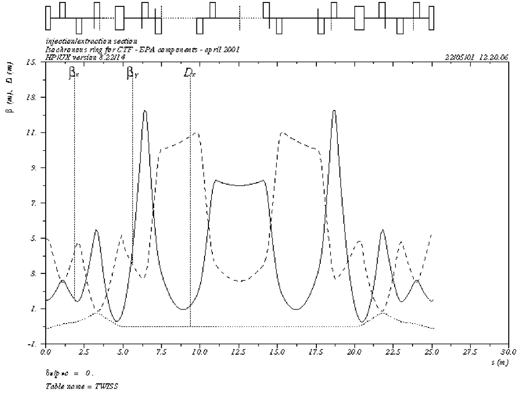
Figure 15.3 Optical functions of injection/extraction from midpoints of adjacent arcs.
