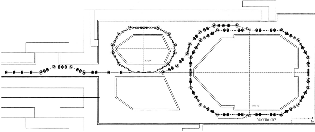
Figure 16.1 CTF3 Layout
