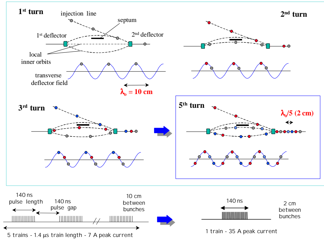
Figure 3.4 Principle of (x5) bunch frequency multiplication
