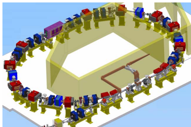
Figure 1: Delay loop layout. The beam comes from the bottom left corner. Septa and dipoles are red, quadrupoles appear in blue. Also visible are the waveguide network feeding the deflector (bottom right) and, on the opposite side, the wiggler (violet).
