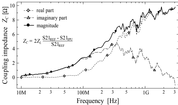
Figure 7: Longitudinal coupling impedance Z_C measured with a coaxial setup of Z_L = 50 \Omega (wire method). For the S21_{REF} reference measurement the IPU was replaced by an equivalent length of a straight tube.
