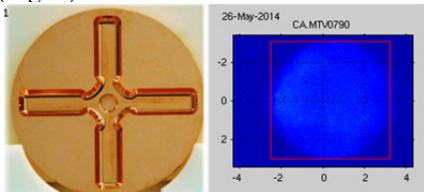
Figure 5: An ACS disk with its 4 HOM damping waveguides and the flat beam collimated by the smallest iris aperture with diameter 4.7 mm.
