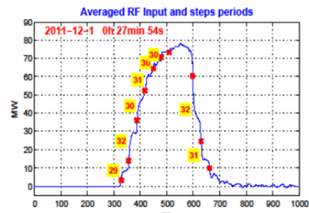
Figure 3: Power pile-up at the PETS output evidencing the recirculation group delay (yellow labels in ns).
