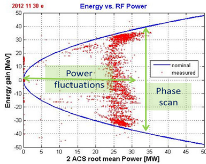
Figure 4: Energy gain obtained with 2 ACS as function of RF phase and power.
