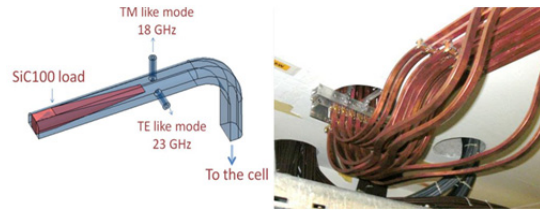
Figure 9: Extended waveguide with the 2 coupling antennas and the SiC absorber and waveguide network to the electronic gallery.
