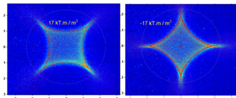
Figure 6: Large beam shape downstream to the ACS at zero crossing, left: towards accelerating phase, right: towards decelerating phase. The red superposed lines are the octupolar model fit.
