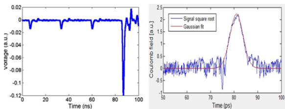
Figure 11: Left: 3 laser pulses though EOS system non synchronous with e^- bunch followed by a synchronous one. Right: spectrum of the chirped laser pulse calibrated in ps corresponding to a bunch length of 6.9 ps FWHM.
