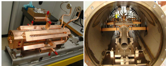
Figure 1: ACS with its WFM waveguide in the middle cell and vacuum test tank with 2 ACS inside.
