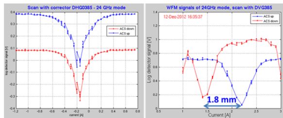
Figure 10: WFM response of the 2 ACS for a horizontal beam position scan (left) and a vertical scan (right). The ACSs were vertically misaligned.
