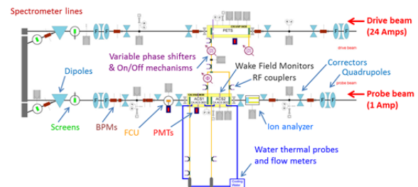
Figure 2: Scheme of the TBTS in CLEX.
